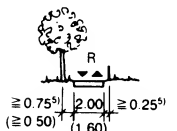
⑥ Separate cycle riders' path
